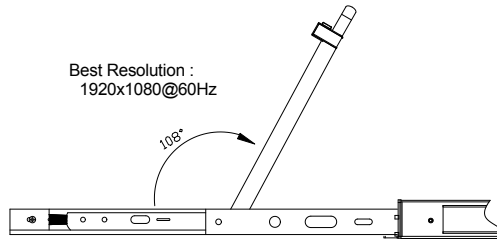
Diagram 1-3.2 open angle of the console
